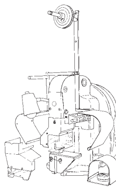
AMP-O-LECTRIC Model "K" Terminating Machine 471273-[] (409-5128)
