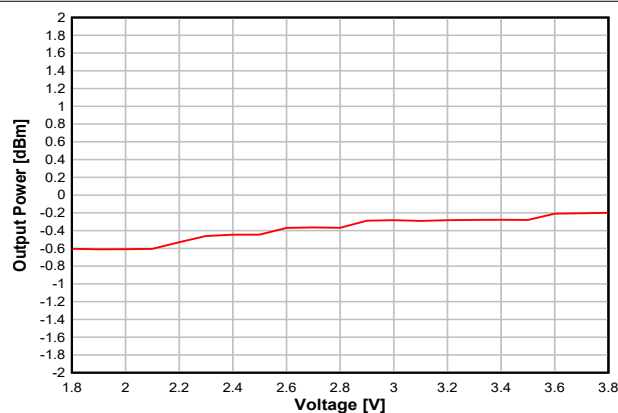
Figure 8-16. Output Power vs. Supply Voltage (VDD) (BLE 1 Mbps, 2.44 GHz, 0 dBm)
