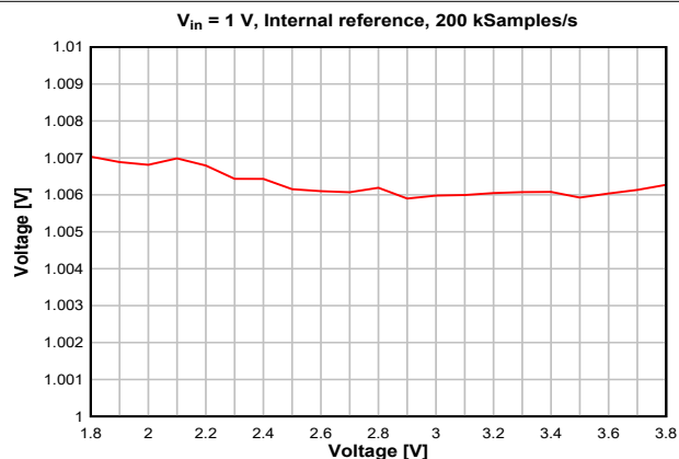
Figure 8-25. ADC Accuracy vs. Supply Voltage (VDD5)
