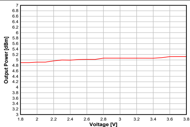
Figure 8-17. Output Power vs. Supply Voltage (VDD) (BLE 1 Mbps, 2.44 GHz, +5 dBm)
