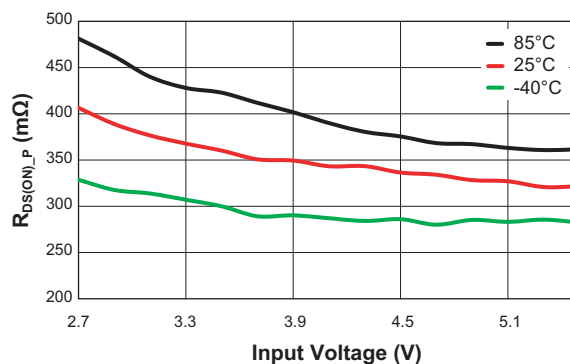
P-Channel R_{DS(ON)} vs. Input Voltage
