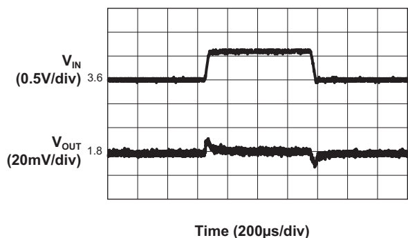
Line Transient
