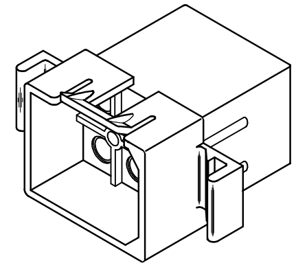
PLUG HOUSING
