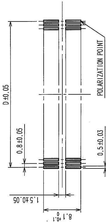
RECOMMENDED P.C.B. LAND PATTERN (MOUNT SIDE)
