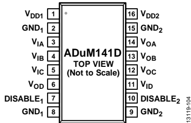
Figure 9. ADuM141D Pin Configuration
