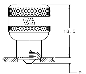
UNFASTENED SCREW PROJECTED
