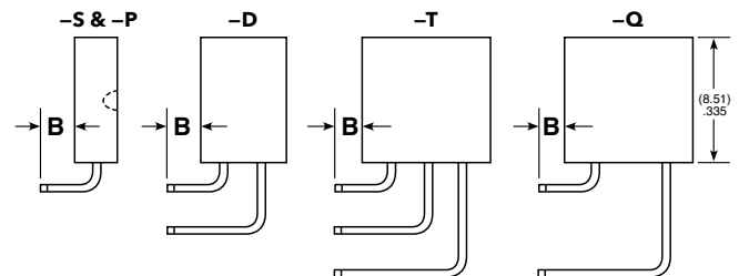
Right-angle Versions
