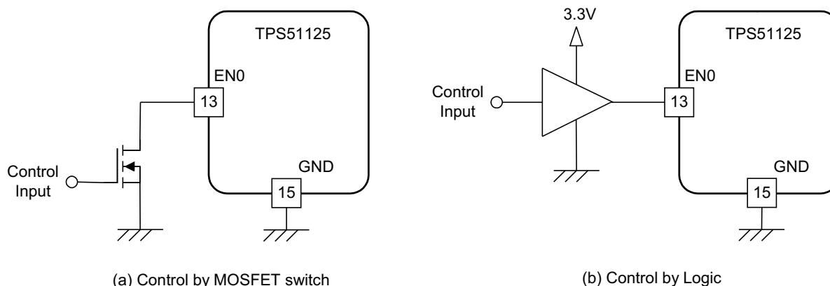
Figure 38. Control Example of EN0 Master Enable
