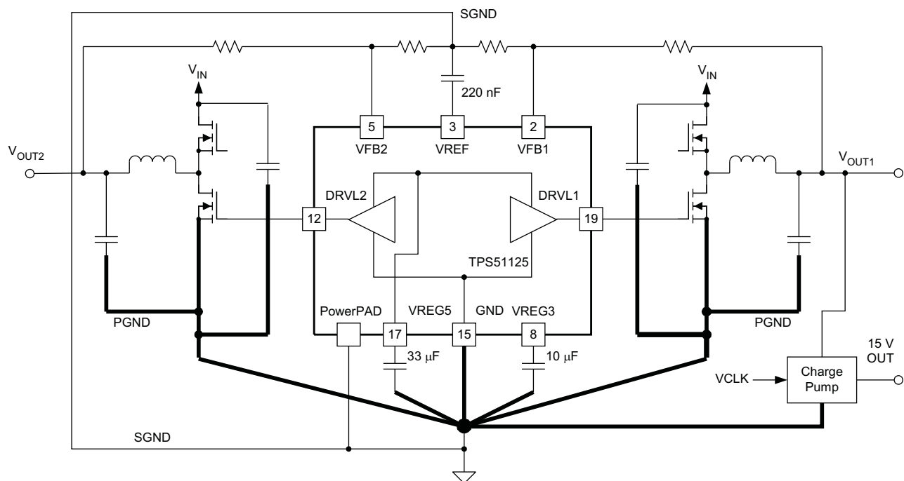
Figure 40. GND system of DC/DC converter using the TPS51125
