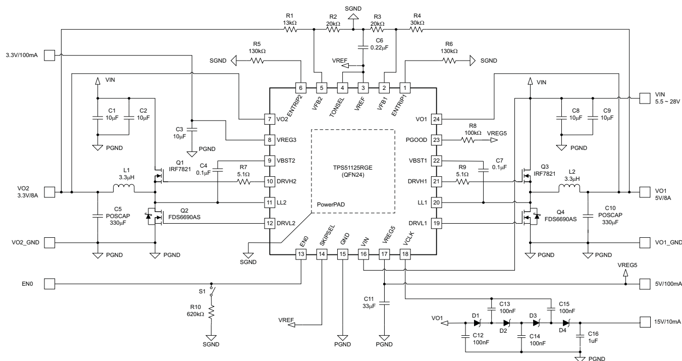
Figure 41. 5-V/8-A, 3.3-V/8-A Application Circuit (245-kHz/305-kHz Setting)
