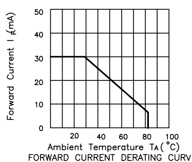
FORWARD CURRENT DERATING CURV
