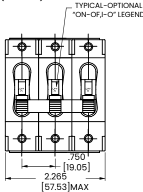
PARALLEL POLE (CA3-P)
