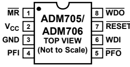
Figure 3.ADM705/ADM706 Pin Configuration
