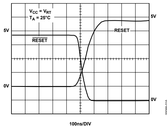
Figure 9. \overline{\text{RESET}} , \overline{\text{RESET}} Assertion
