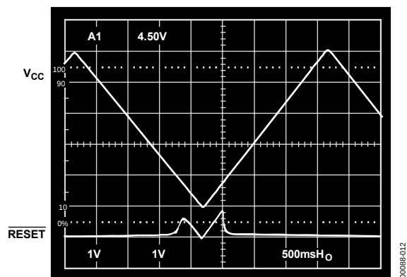
Figure 5. \overline{\text{RESET}} Output Voltage vs. Supply Voltage
