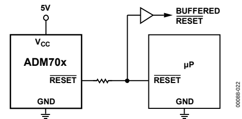
Figure 20. Bidirectional I-O RESET
