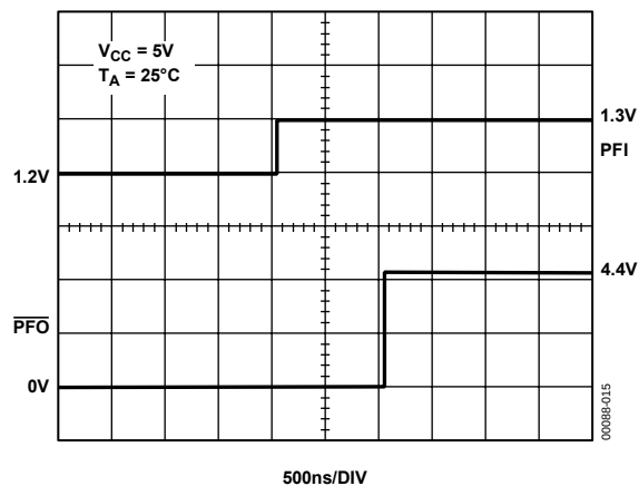
Figure 8. PFI Comparator Deassertion Response Time
