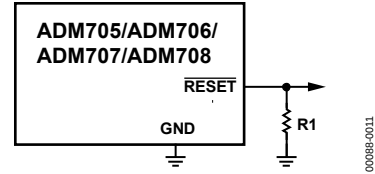
Figure 16. RESET Valid Below 1 V
