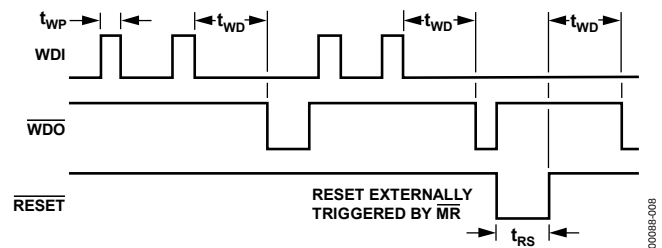
Figure 13. Watchdog Timing
