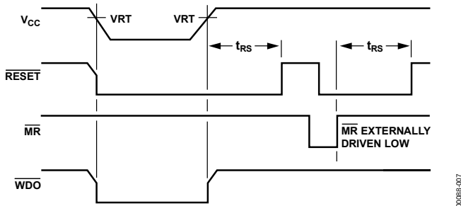
Figure 12. \overline{\text{RESET}} , \overline{\text{MR}} , and \overline{\text{WDO}} Timing
