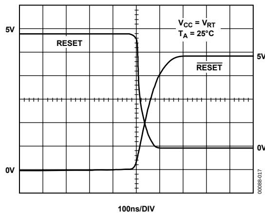
Figure 10. \overline{\text{RESET}} , \overline{\text{RESET}} Deassertion
