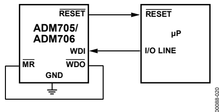
Figure 18. RESET from WDO
