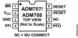
Figure 4.ADM707/ADM708 Pin Configuration
