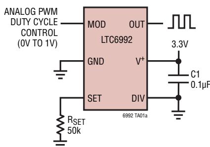
1MHz Pulse Width Modulator
