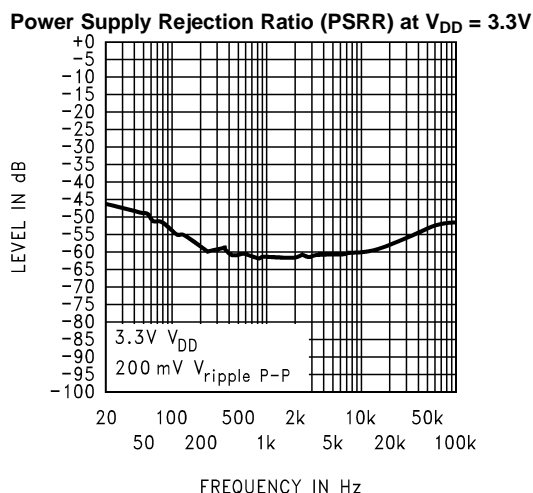
Figure 17. Input terminated with 10\Omega R
