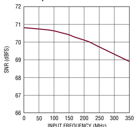
LTC2264-12: SNR vs Input Frequency, -1\text{dBFS} , 2\text{V} Range, 40\text{Mpsps}
