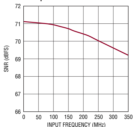
LTC2265-12: SNR vs Input Frequency, -1\text{dBFS} , 2\text{V} Range, 65\text{Mps}
