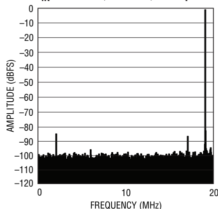
LTC2264-12: 8k Point FFT, f_{IN} = 139\text{MHz} , -1\text{dBFS} , 40\text{Mpsps}
