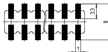
PCB layout
