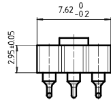
Dimensions of Pick-and-Place pad for 3 pole strip
