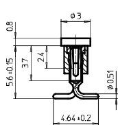
Dimensions of Pick-and-Place pad for 3 pole strip
