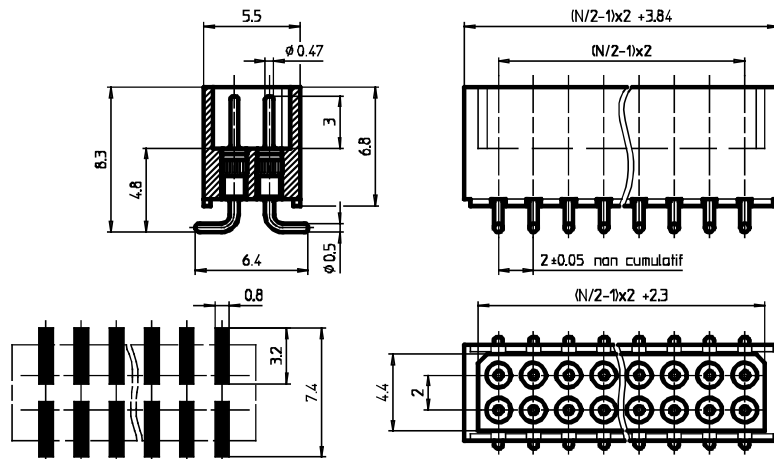
PCB layout
