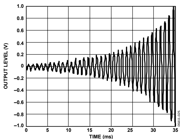
Figure 25. Slew RAM—Constant dB Update Increasing Ramp
