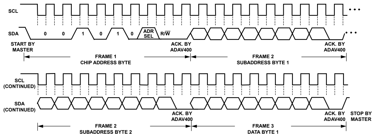
Figure 20. I²C Write Format
