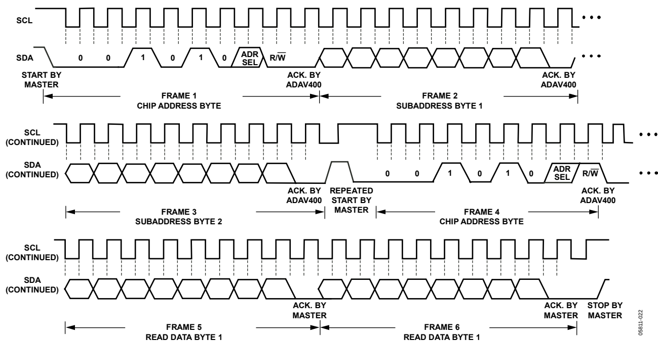
Figure 21. I²C Read Format
