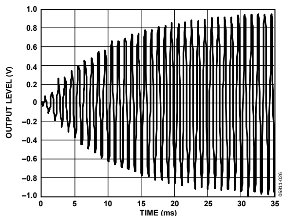
Figure 26. Slew RAM—RC Update Increasing Ramp
