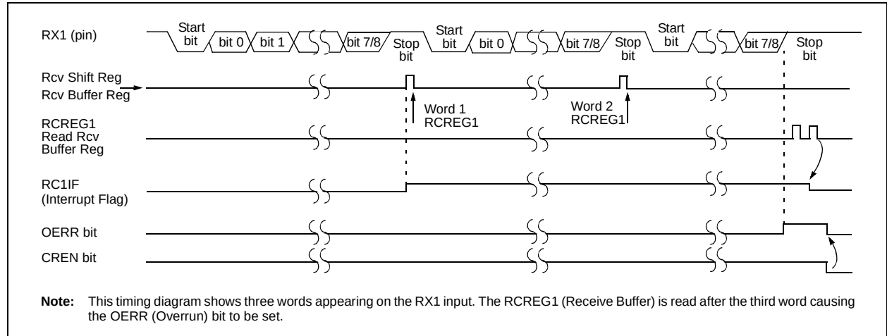
FIGURE 17-7: ASYNCHRONOUS RECEPTION
