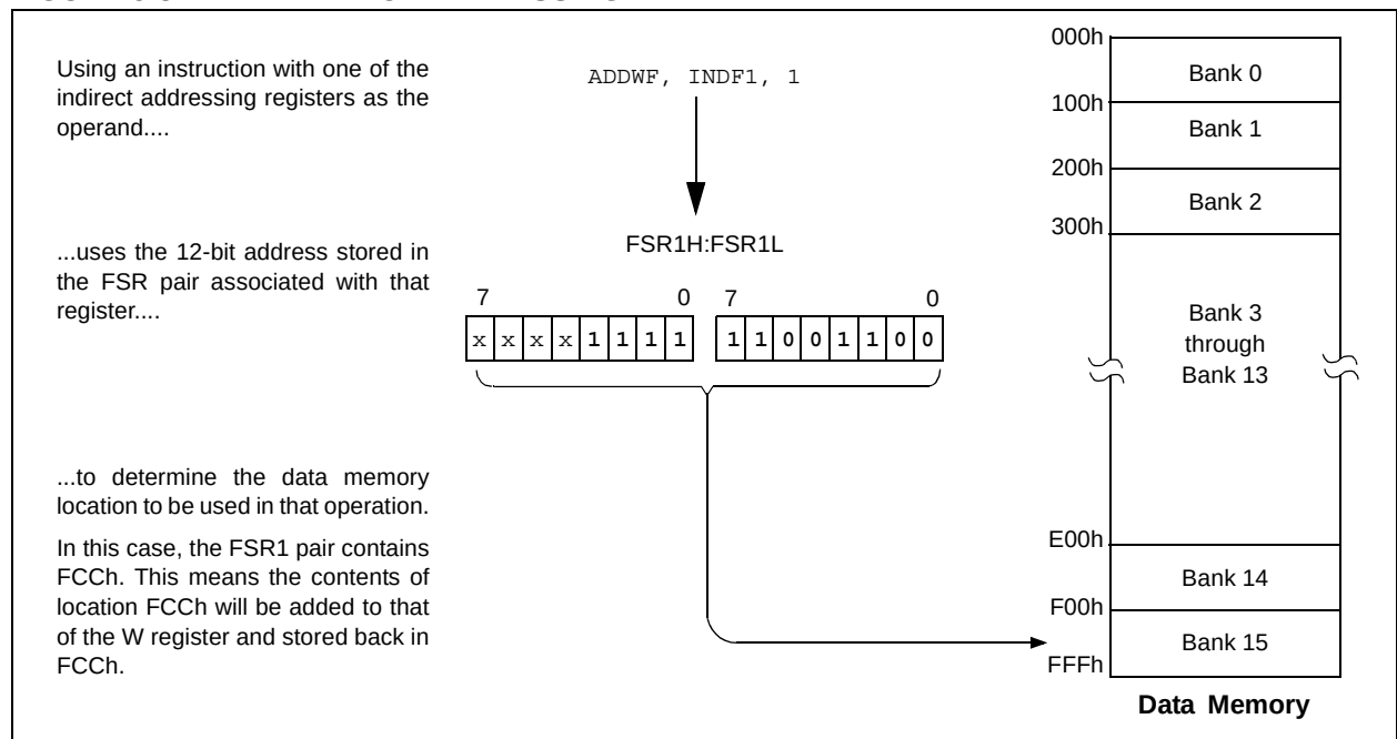
FIGURE 5-8: INDIRECT ADDRESSING
