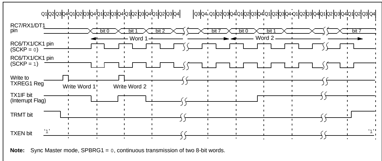
FIGURE 17-11: SYNCHRONOUS TRANSMISSION
