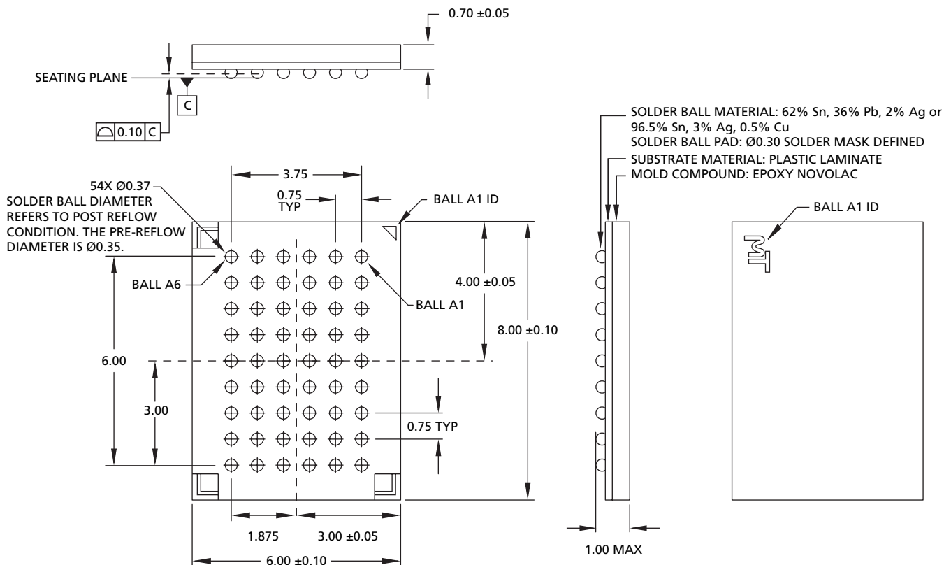
Figure 49: 54-Ball VFBGA
