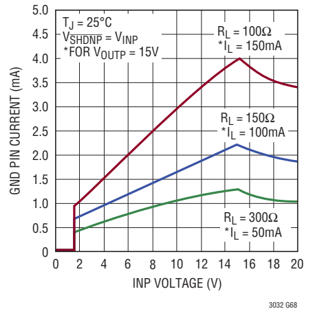
LT3032-15 Positive Side GND Pin Current
