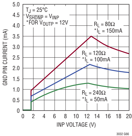
LT3032-12 Positive Side GND Pin Current
