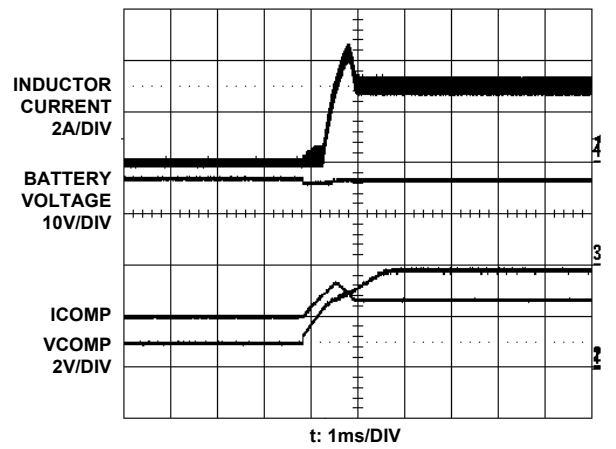
FIGURE 10. BATTERY INSERTION
