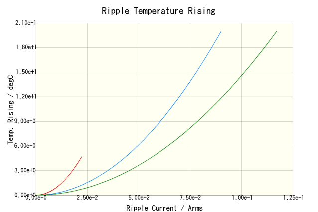
C1608X7R2A102K080AA(100kHz) C1608X7R2A102K080AA(500kHz) C1608X7R2A102K080AA(1MHz)
