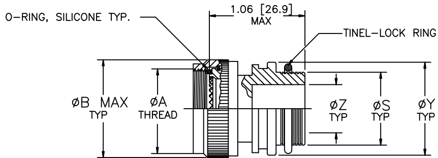
FIGURE 1 STRAIGHT ADAPTER
