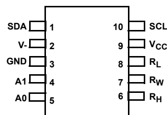
ISL23711 (10 LD MSOP) TOP VIEW
