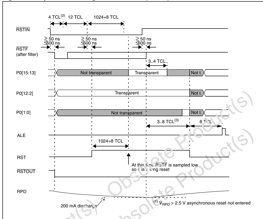
Figure 82. Synchronous long hardware reset ( \overline{\text{EA}} = 0 )
