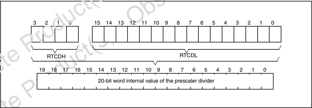
Figure 74. Divider counter registers
