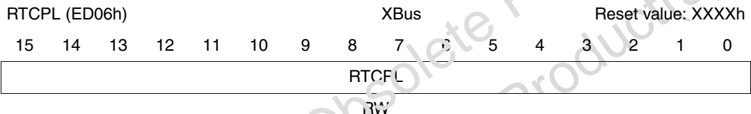
Figure 73. Prescaler registers
