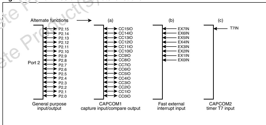
Figure 53. Port 2 I/O and alternate functions
