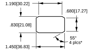
MOUNTING HOLE (Nylon Snap-in Brackets)
