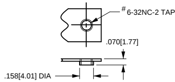
TAPPED HOLE Standard with A & B Brackets
