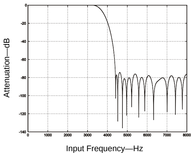
Figure 4. FIR Transmit Filter Response
