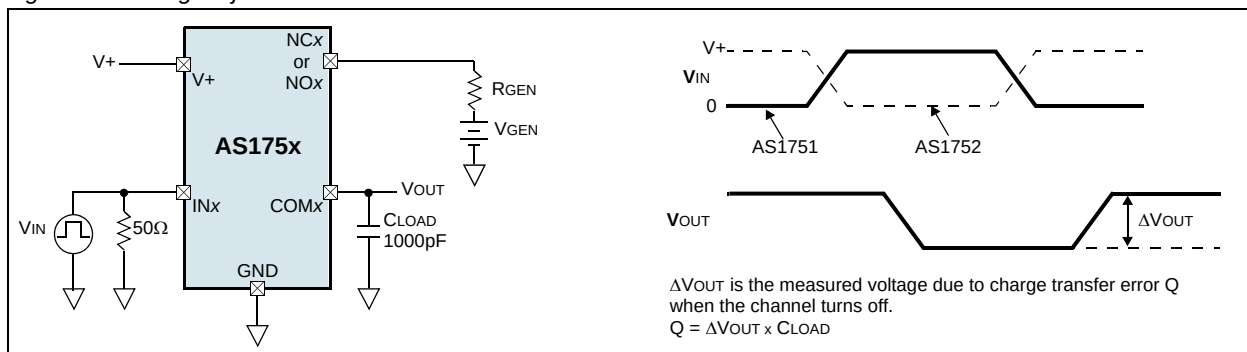
Figure 16. Charge Injection
