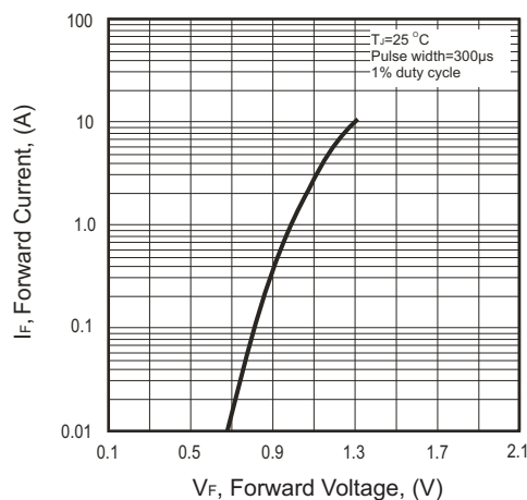
Fig.2- Forward Characteristics
