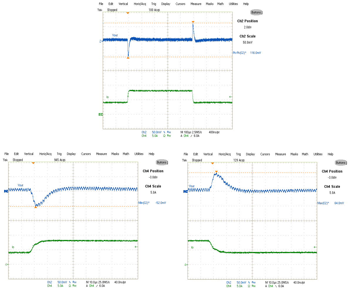
Fig. 23: Transient Response, 4A to 8A step 2.5A/μs Ch_2: V_{out} , Ch_4: I_{out}
