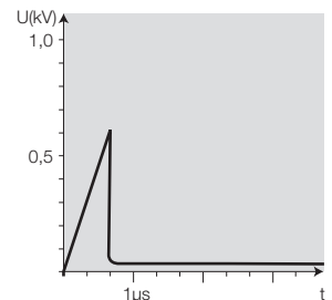
Pulse form shape with GDT
