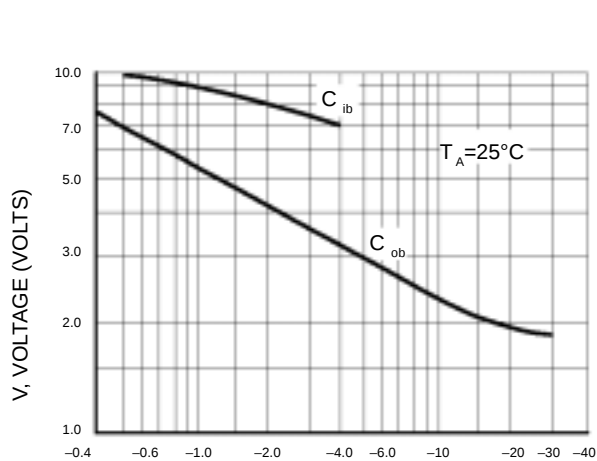
V_R , REVERSE VOLTAGE (VOLTS) Figure 5. Capacitances
