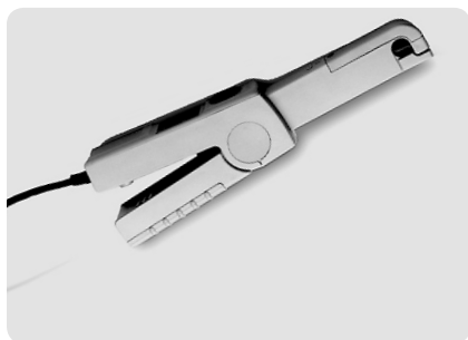
1146B 100 mA to 100 Arms, dc to 100 kHz probe.
