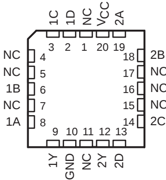
54ACT11020 . . . FK PACKAGE (TOP VIEW)
