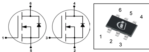
PG-TSOP-6
