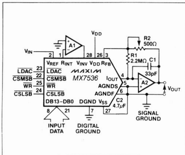
Figure 4. MX7536 Operation
