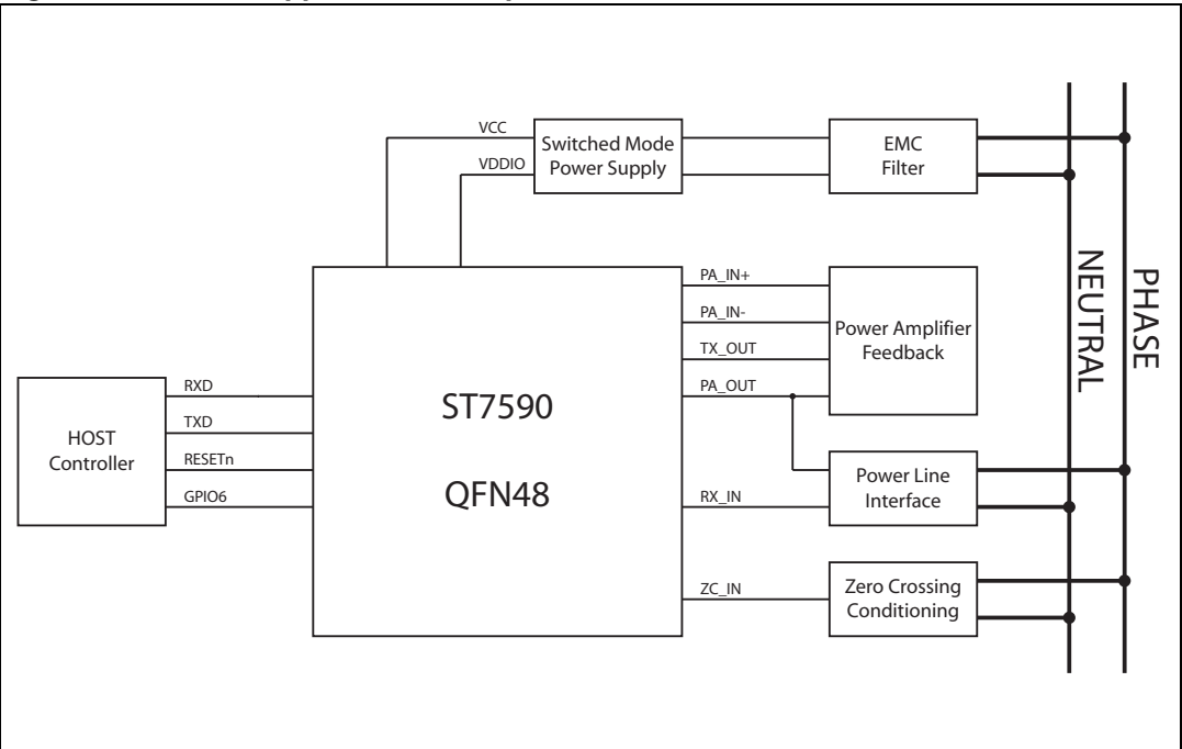
Figure 9. QFN48 application example
