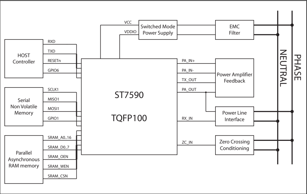
Figure 8. TQFP100 128 Kb external memory application example
