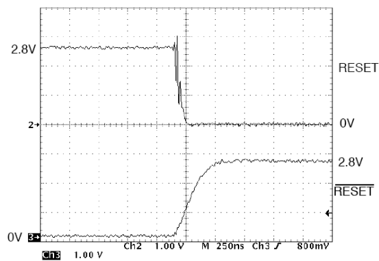
Fig. 13: SP708 RESET and RESET De-Assertion
