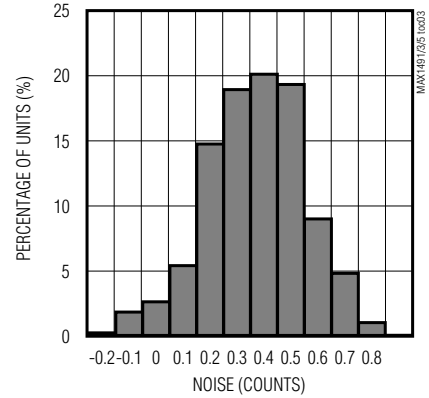
NOISE DISTRIBUTION
