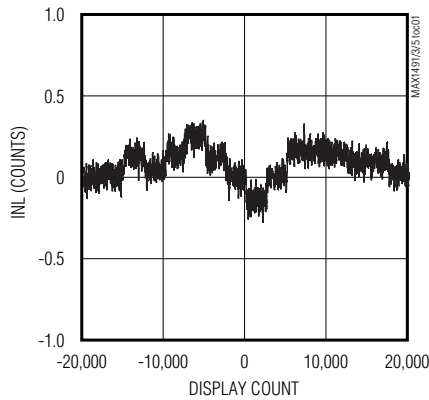
MAX1493/MAX1495 ( \pm 200mV INPUT RANGE) INL vs. DISPLAY COUNT
