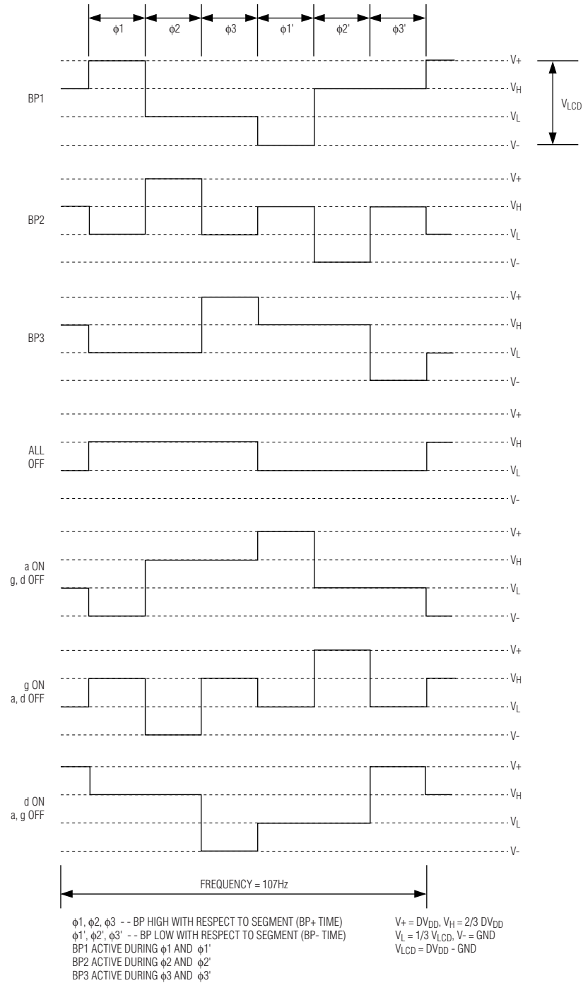
Figure 9. LCD Voltage Waveform—Combinations 1–4 (BP1/2/3, SEGa/d/g)
