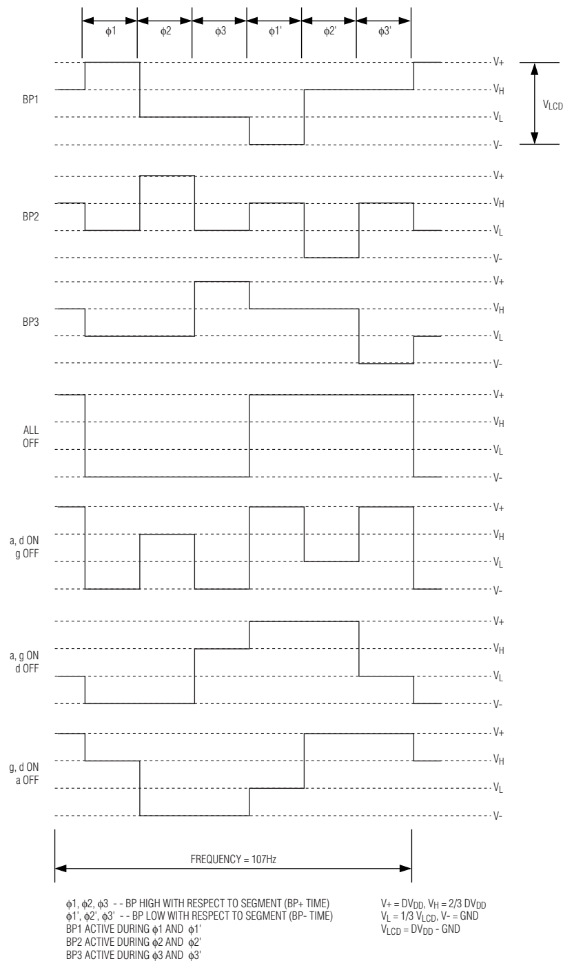
Figure 10. LCD Voltage Waveform—Combinations 5–8 (BP1/2/3, SEGa/d/g)
