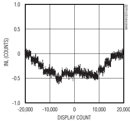
MAX1493/MAX1495 ( \pm 2V INPUT RANGE) INL vs. DISPLAY COUNT
