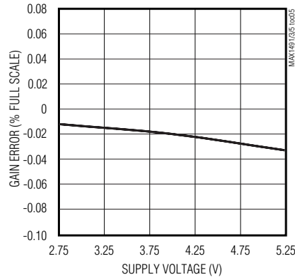
MAX1493/MAX1495 GAIN ERROR vs. SUPPLY VOLTAGE
