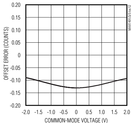
OFFSET ERROR vs. COMMON-MODE VOLTAGE
