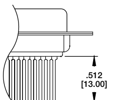
Wire Wrap Tail Option Tail length 2 wire wrap tail
