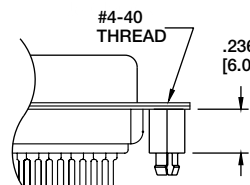
BL Option #4-40 Threaded Boardlocks
