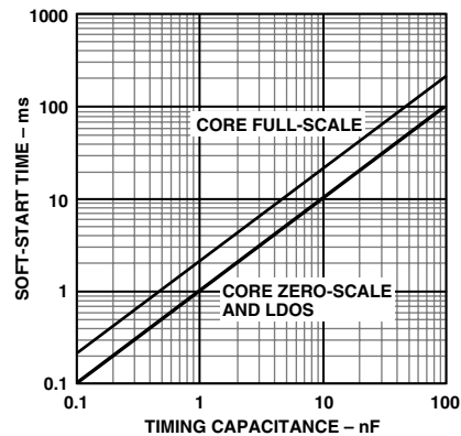
TPC 3. Soft-Start Time vs. Timing Capacitance
