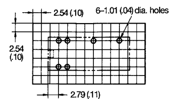
Mounting holes
