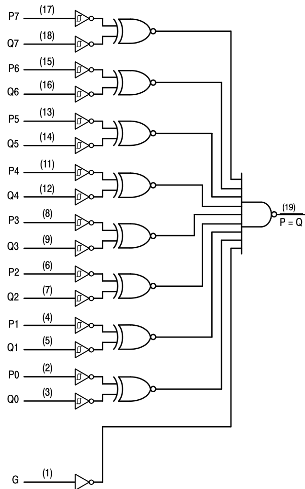
SN54/74LS688
