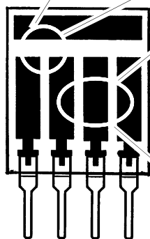
SIP PINS ON .100 in. Centers
