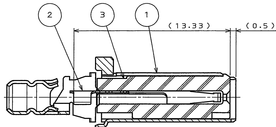
SECT. A-A
