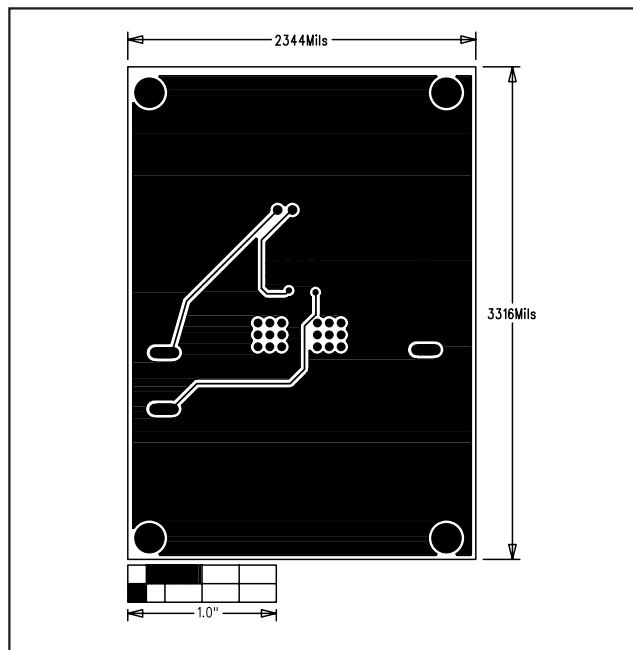
Figure 5. MAX8556 EV Kit PC Board Layout—Layer 3
