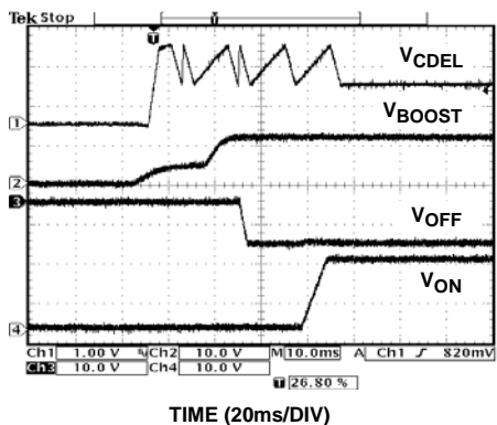
FIGURE 11. START-UP SEQUENCE
