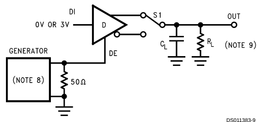
FIGURE 8. Driver TRI-STATE Test Circuit ( t_{PZH} , t_{PHZ} )
