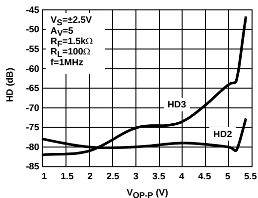
FIGURE 8. DIFFERENTIAL HARMONIC DISTORTION vs DIFFERENTIAL OUTPUT VOLTAGE (ALL PACKAGES)
