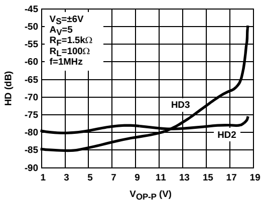
FIGURE 10. DIFFERENTIAL HARMONIC DISTORTION vs DIFFERENTIAL OUTPUT VOLTAGE (ALL PACKAGES)
