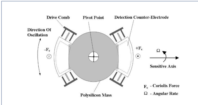
Fig. 1: Basic layout of the sensing element of SMG061
